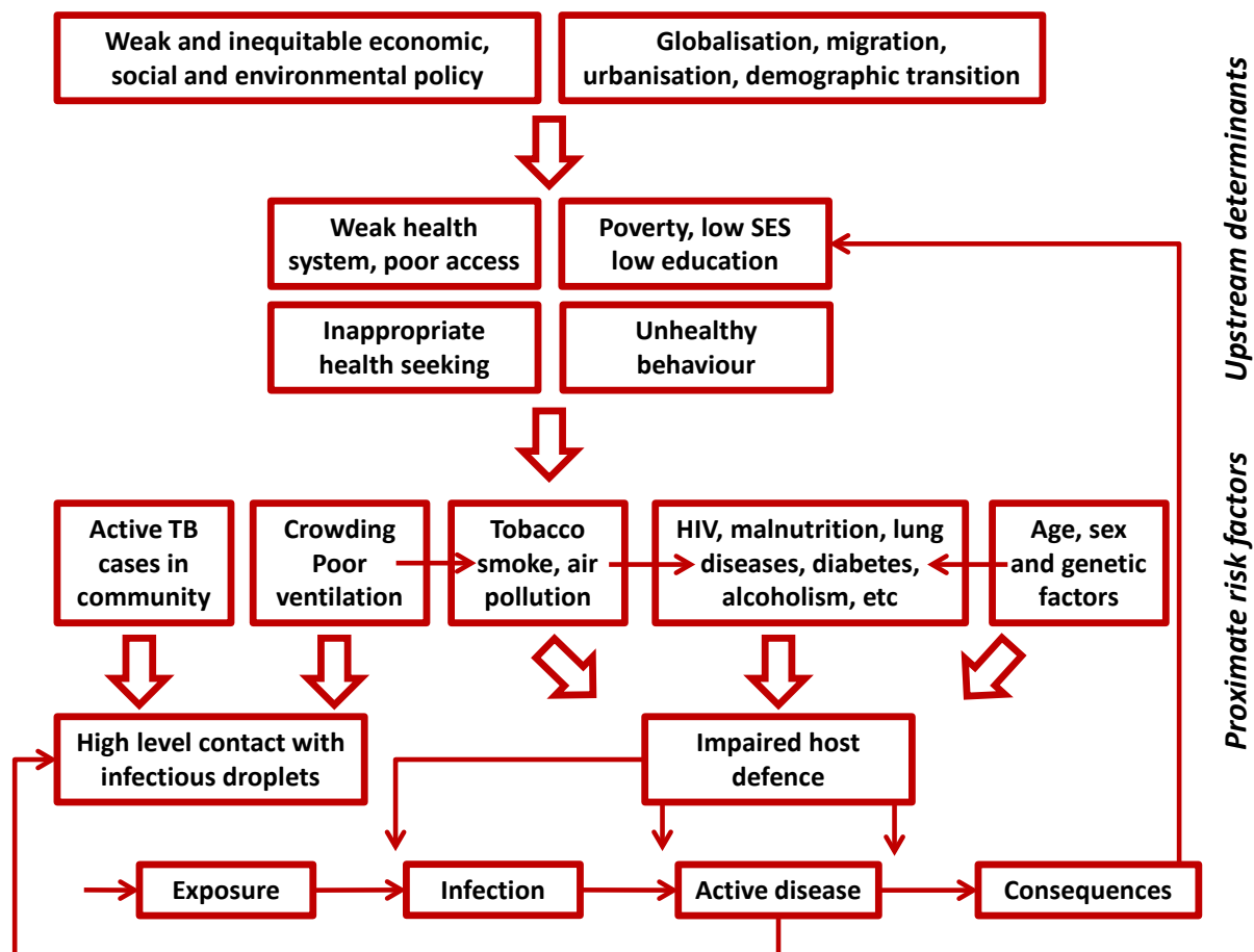
Figure 2. Framework for proximate risk factors and upstream determinants of TB 39
